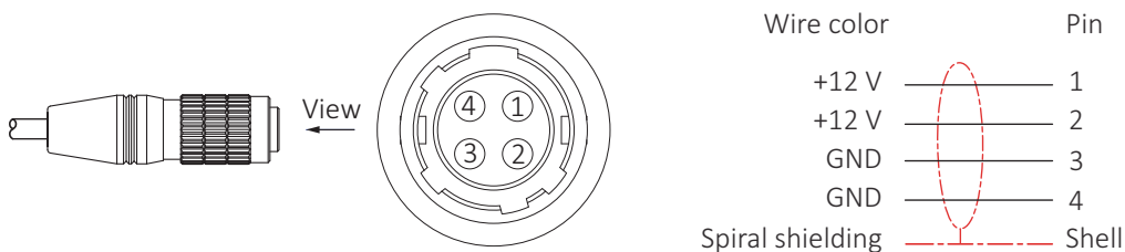
Figure 2: Output connector pin assignment and wiring diagram
