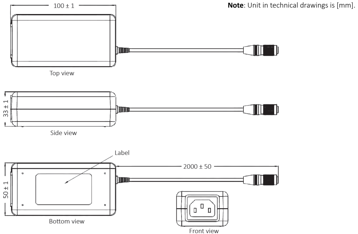
Figure 1: Power supply and output cable dimensions
