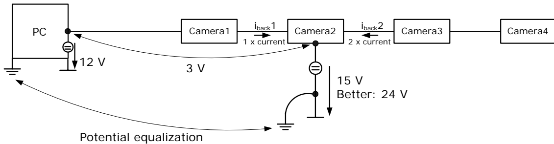
Fig. 4: Scenario with more than 3 cameras
