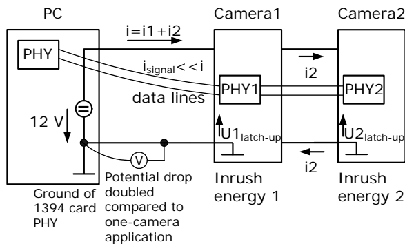
Fig. 1: Two camera scenario with power from PC
