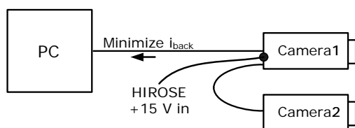
Fig. 2: Schema of Daisy Chaining and HIROSE
