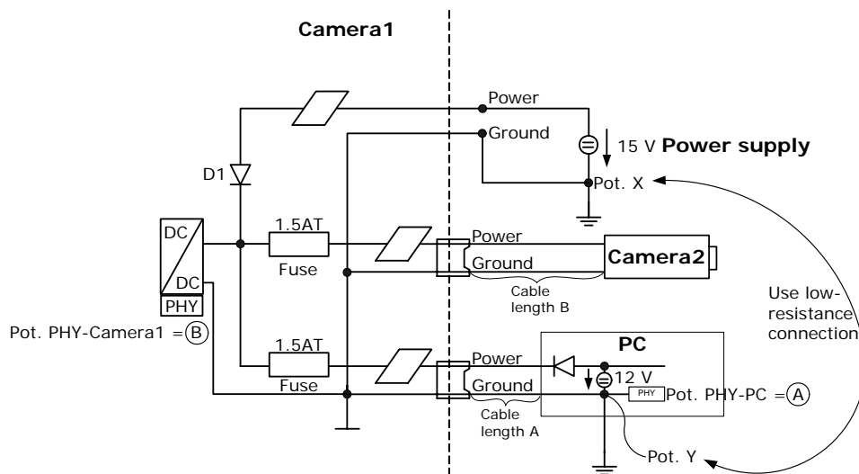
Fig. 3: Details of Daisy Chaining and HIROSE
