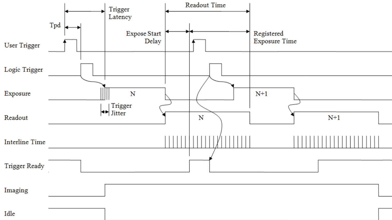
Figure 18: Prosilica GS internal signal timing waveforms
