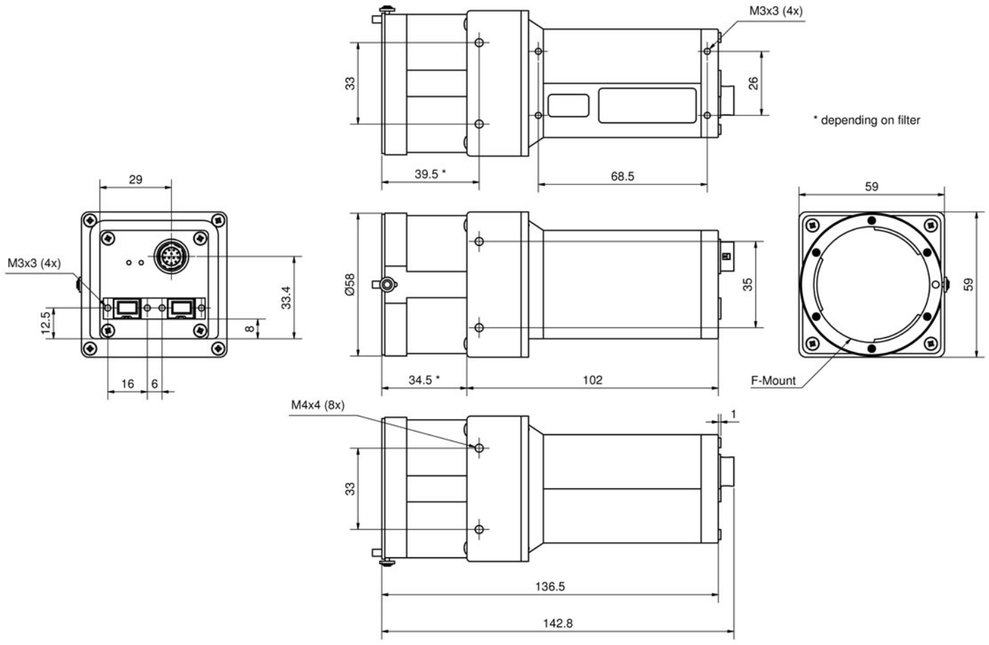
Pike F-Mount (2x IEEE1394b) 142.8 x 59 x 59 (L x W x H)
