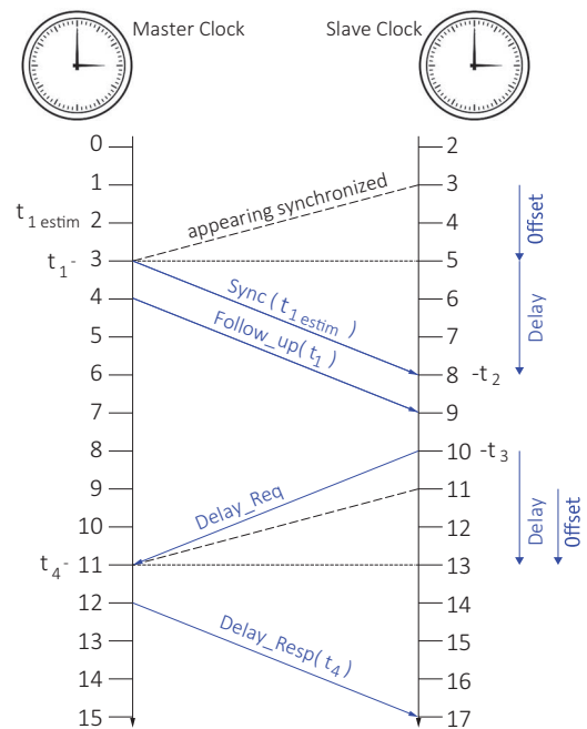
Figure 1: Multicast sync packets
