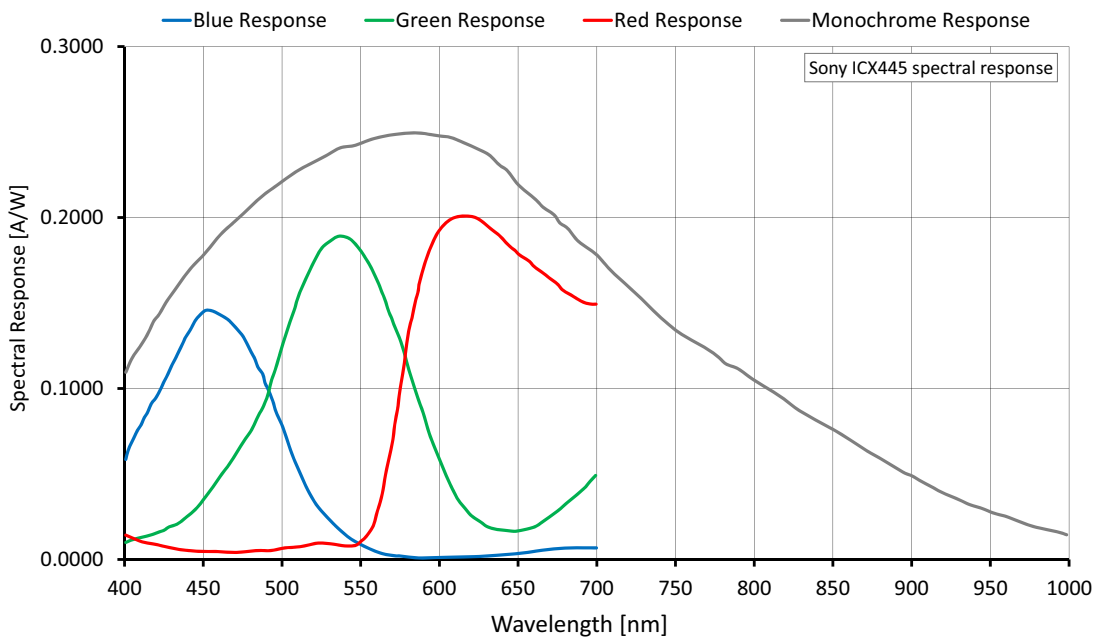
Figure 9: Mako G-125 (Sony ICX445) spectral response
