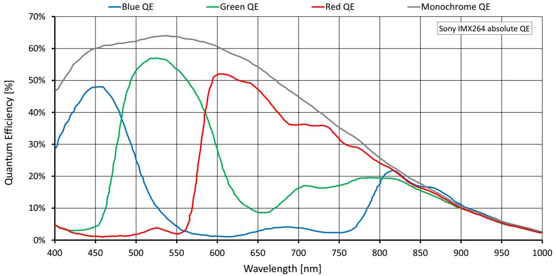
Figure 38: Mako G-507 (Sony IMX264) absolute QE
