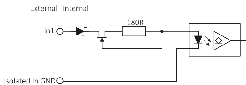
Figure 69: Input block diagram
