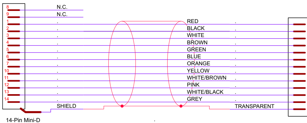
Figure 13: Prosilica GB/GS cable color-coding
